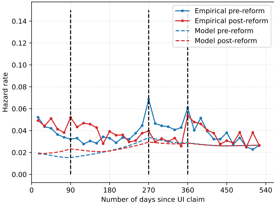
Initial fit — Reference dependent 1 type (L-BFGS-B)
